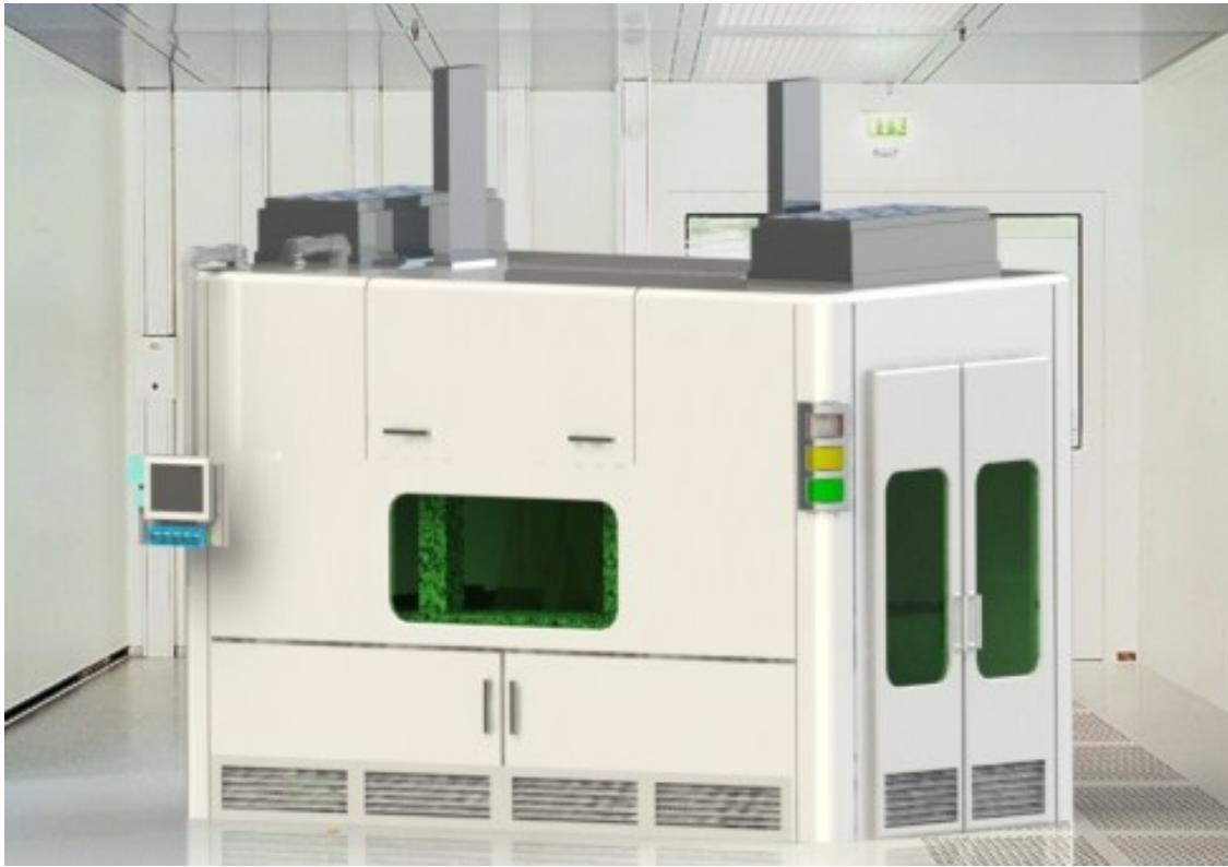
TC film (ITO, AgNW) and silver paste patterning tool
