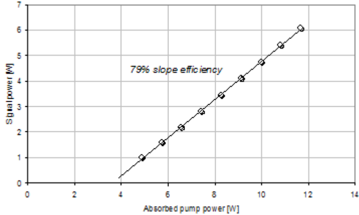
Typical performance data for Yb1200-25/250DC-PM
