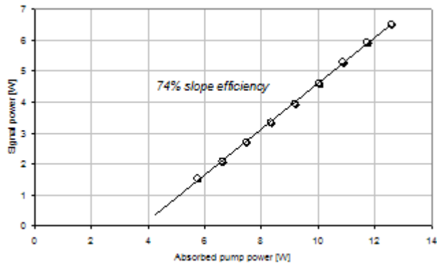
Typical performance data for Yb1200-25/250DC-PM
